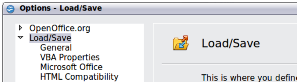
Figure 18: Load/Save options
