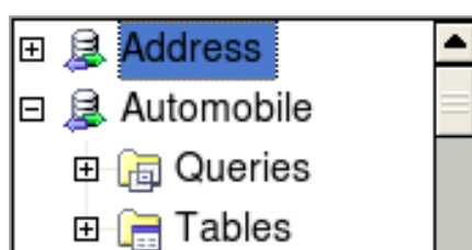
Figure 36: Databases
