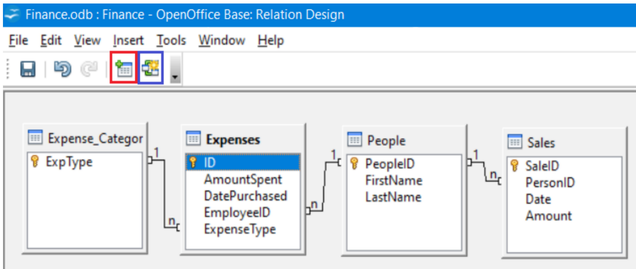
Figure 166: Designation for a 1:n relationships
