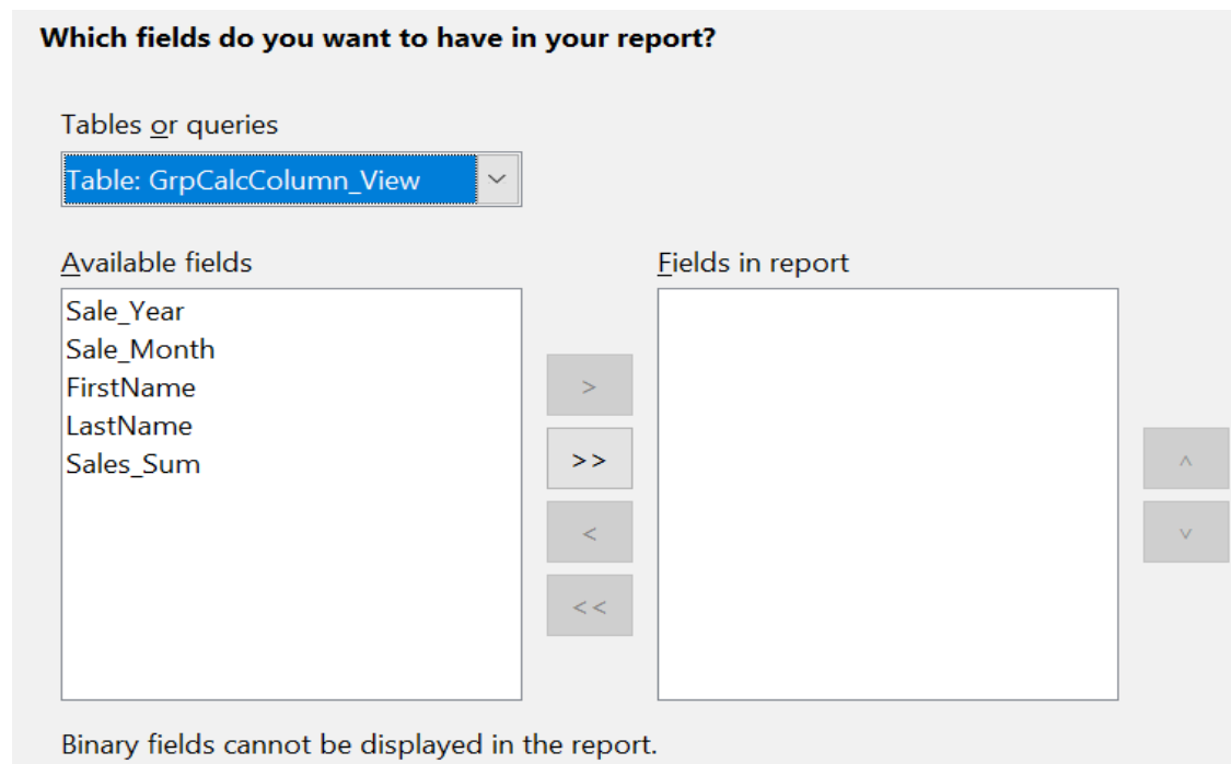
Figure 199: Dialog for choose the fields in a report.
