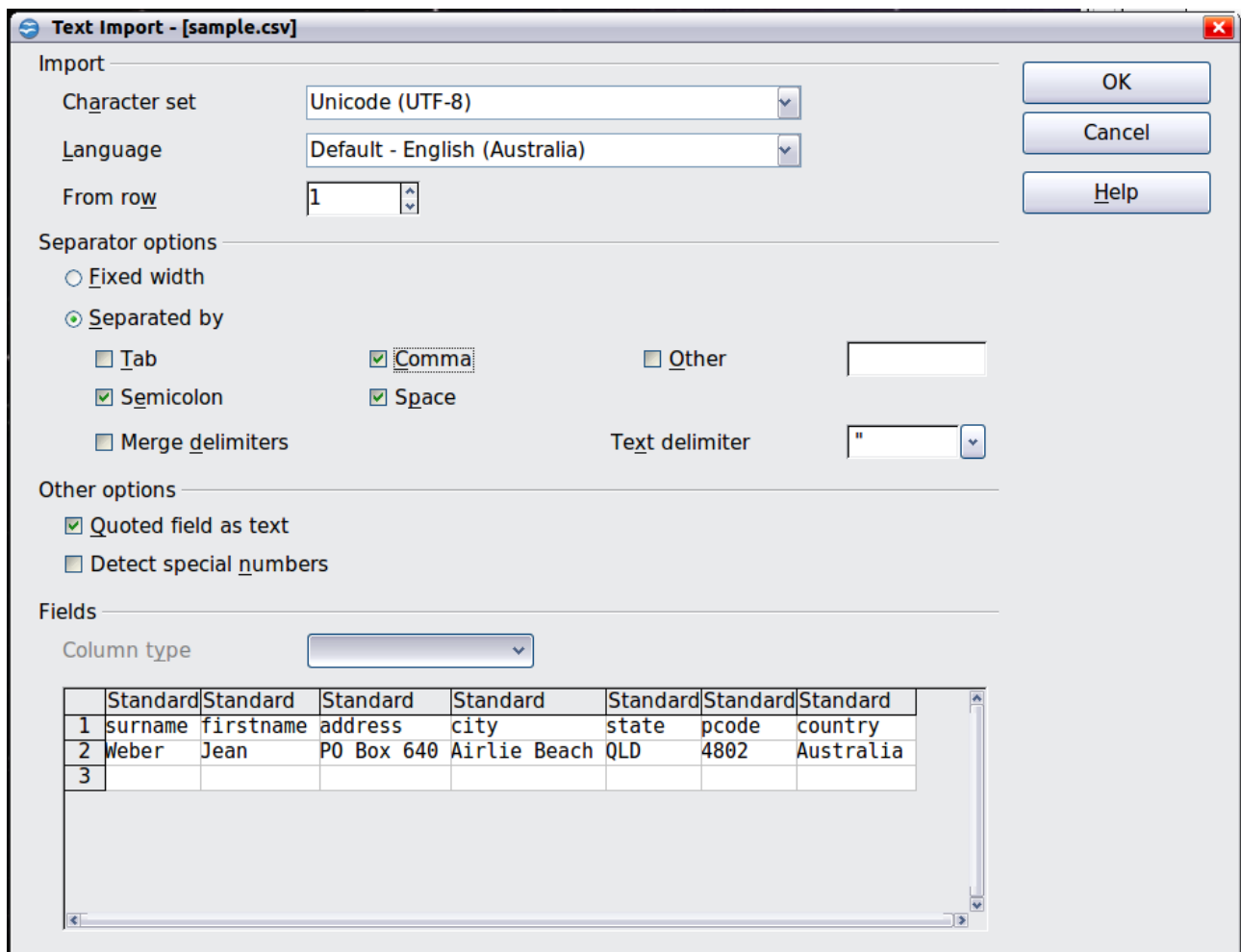
Figure 6: Text Import dialog, with Comma (,) selected as the separator and double quotation mark (") as the text delimiter.
