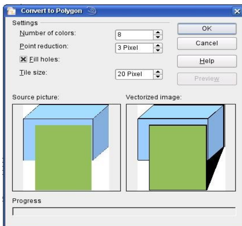
Figure 124: Conversion of a picture to polygons
