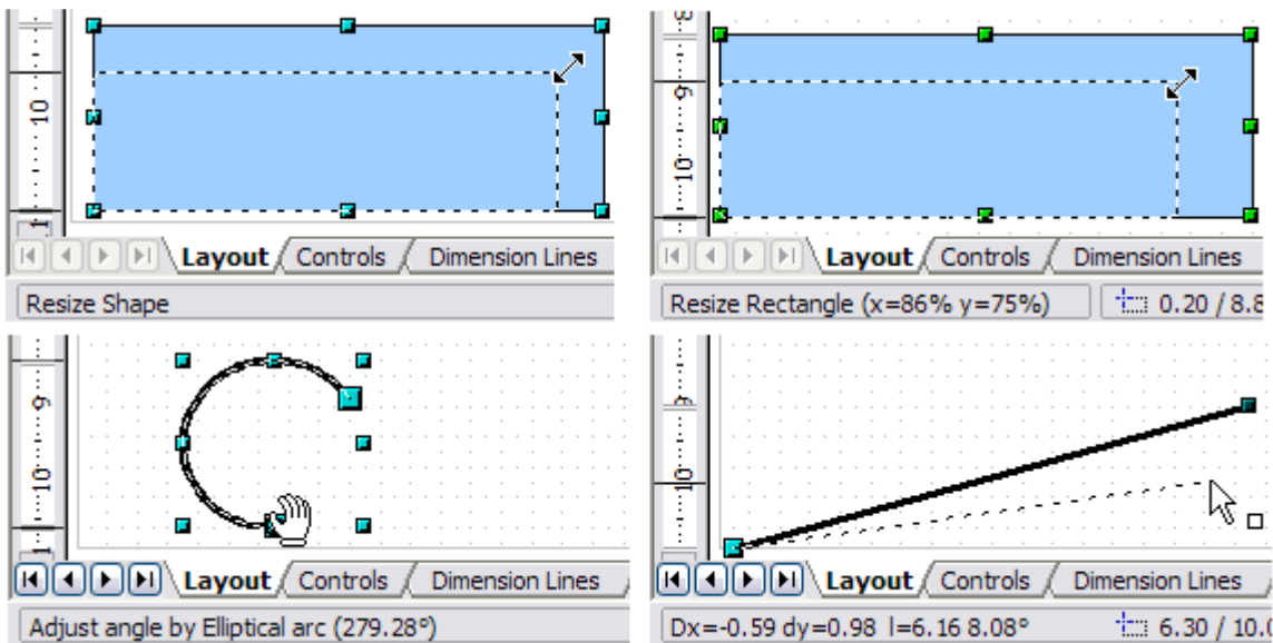
Figure 38: The Information field during dynamic size modification of objects
