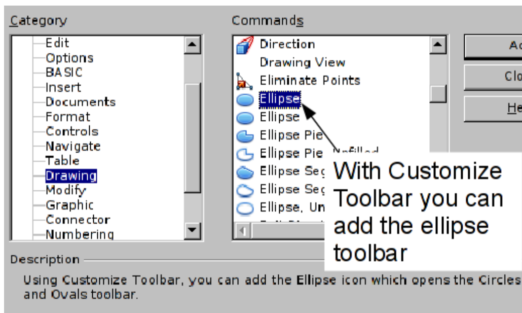
Figure 23: Adding the extended Ellipse toolbar
