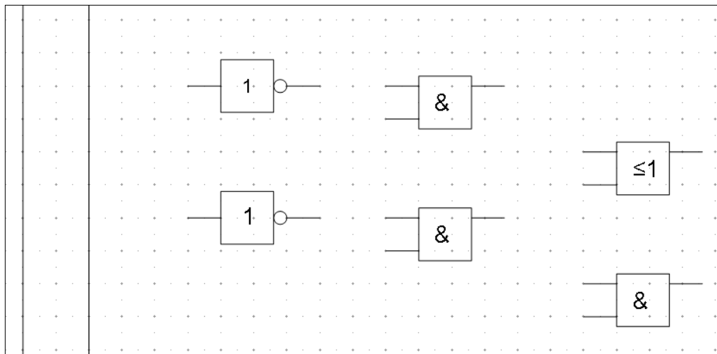
Figure 225: Drawing a half adder - Step 3
