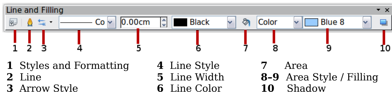
Figure 64: Line and Filling toolbar
